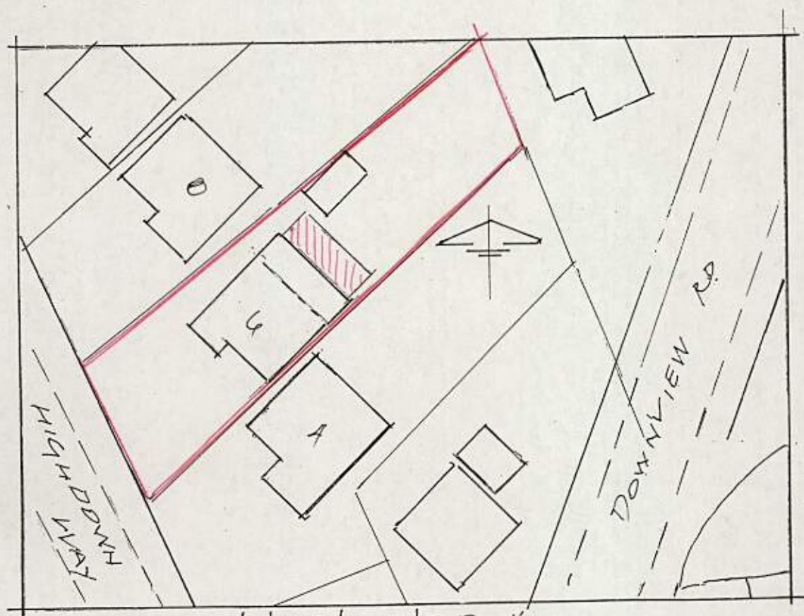
block plan \frac{1}{500}
