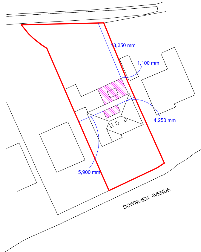
SITE/ROOF PLAN - 1/500
