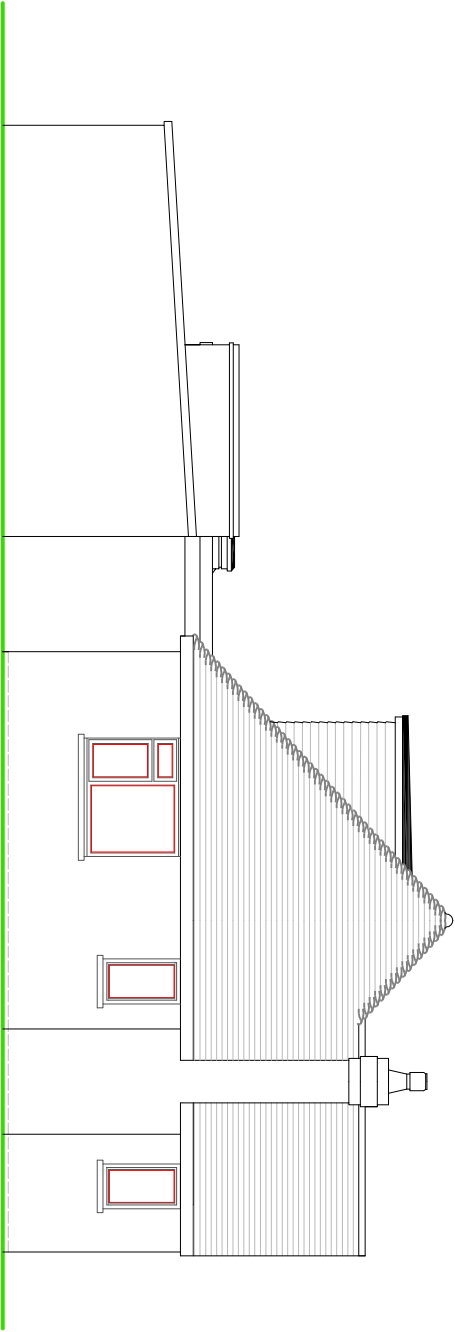
SIDE ELEVATION
