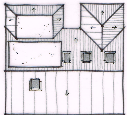
ROOF PLAN 1:200
