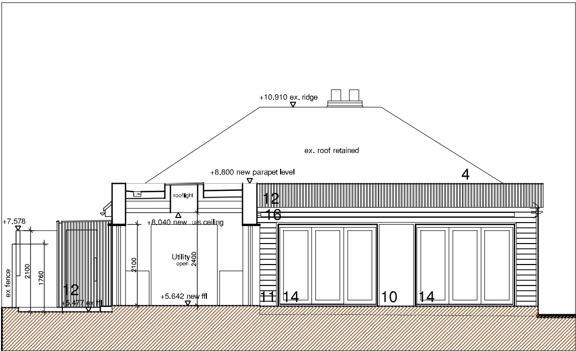
1:100 North elevation as proposed
