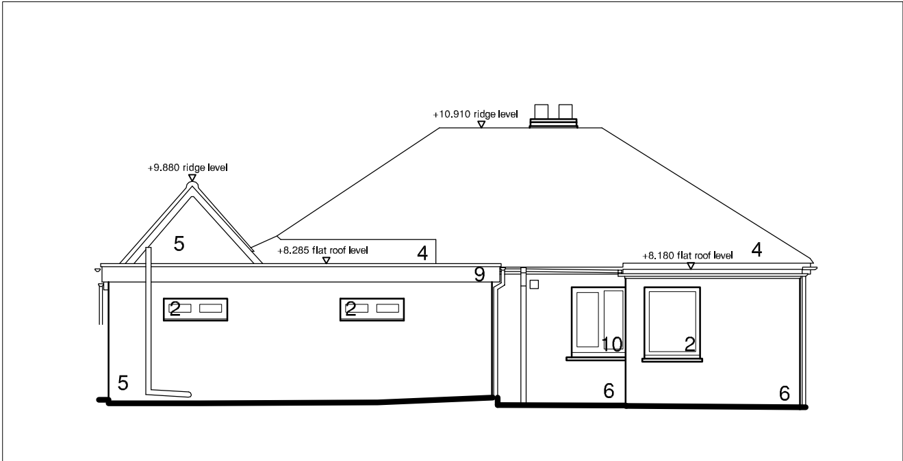
1:100 North Elevation as existing
