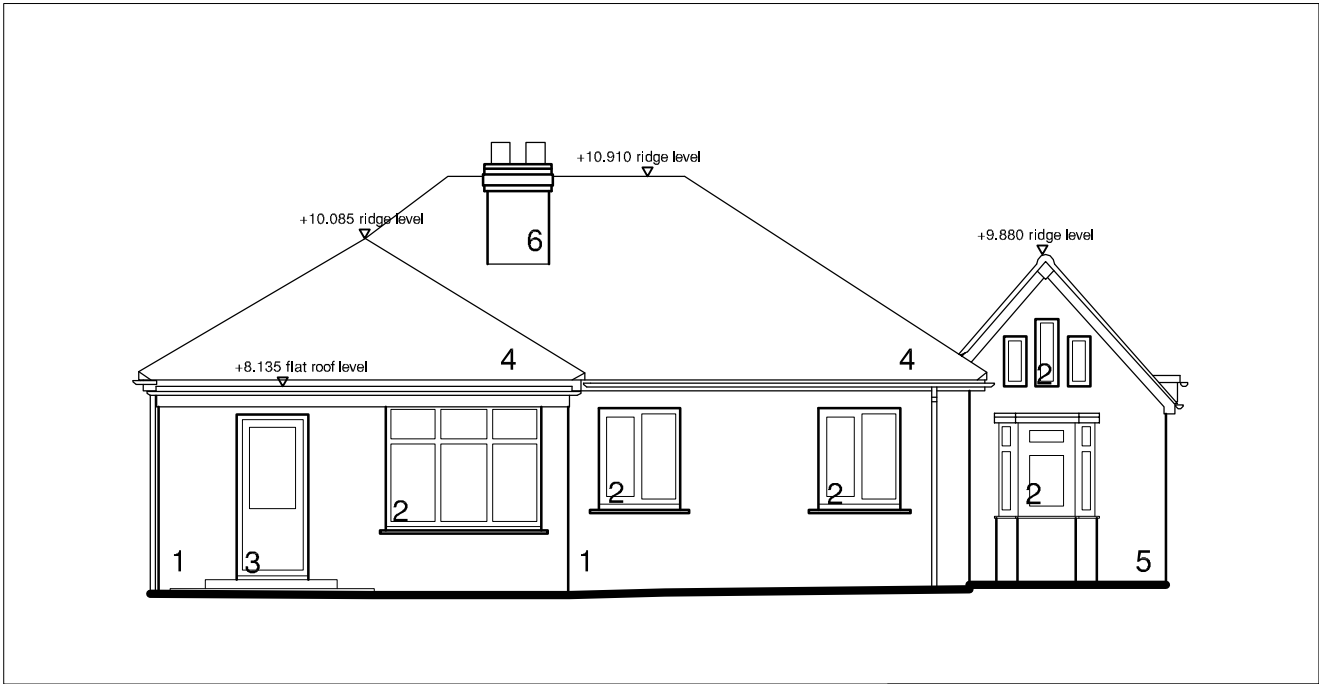
1:100 South Elevation as existing
