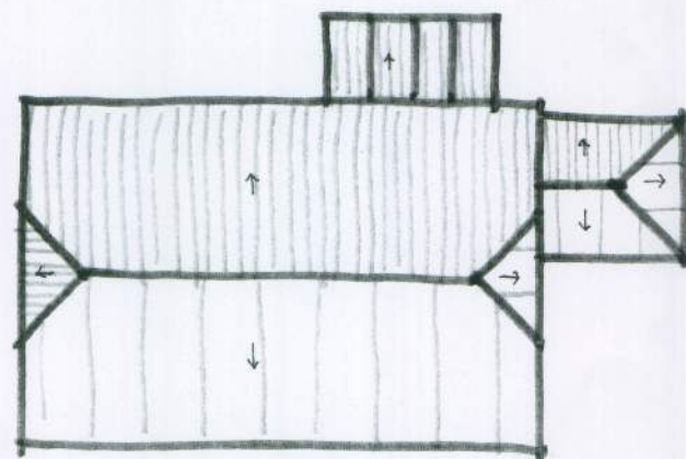
ROOF PLAN 1:200
