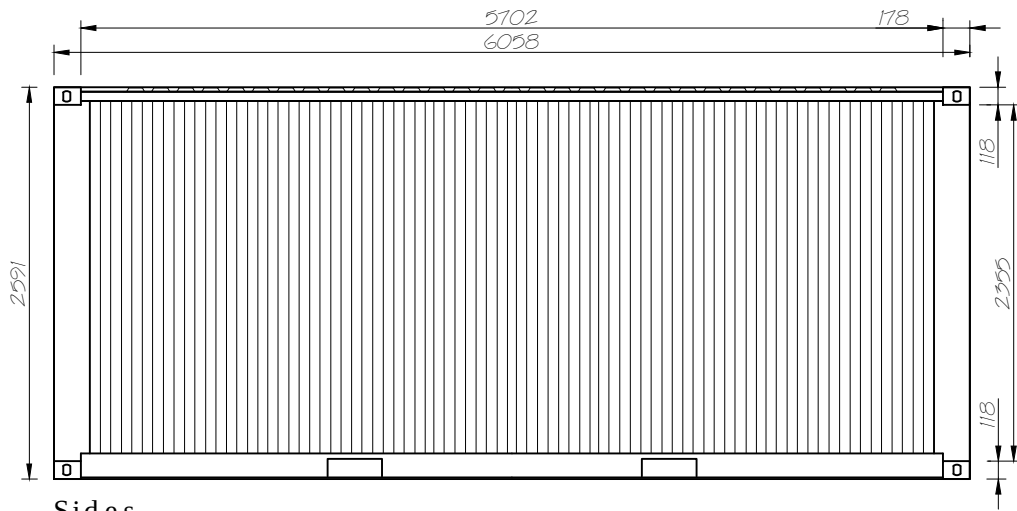
Sides
