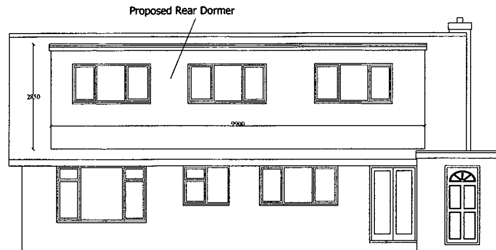
Rear Elevation (North)
