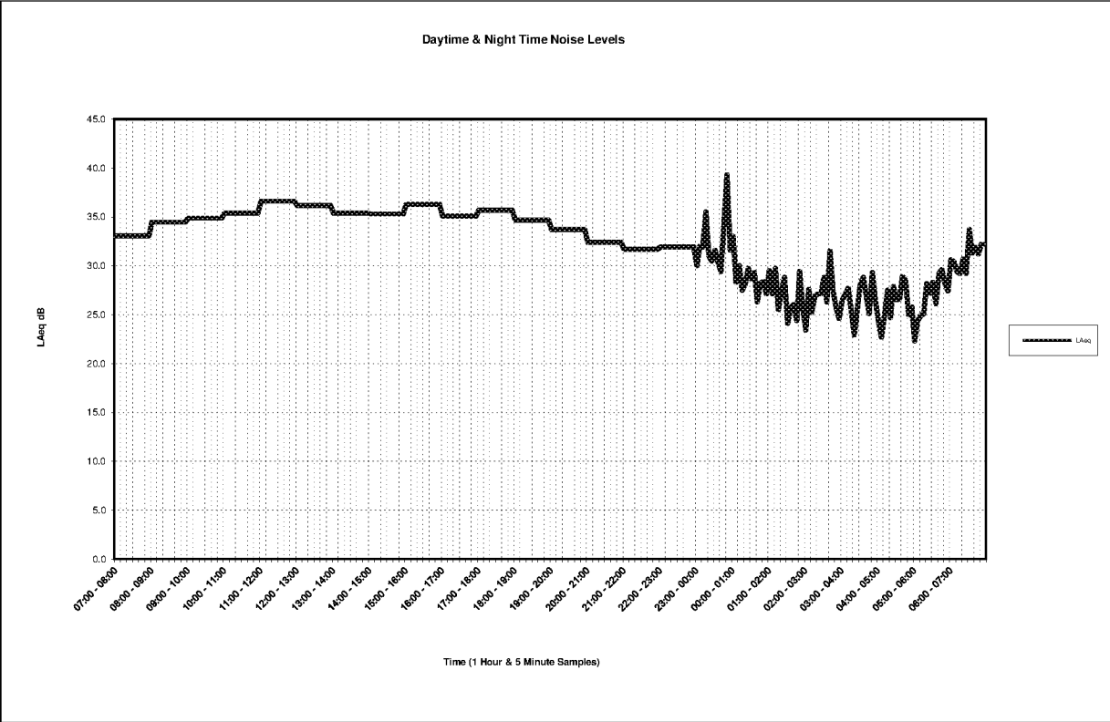
DAYTIME NOISE LEVELS 07:00 - 23:00
