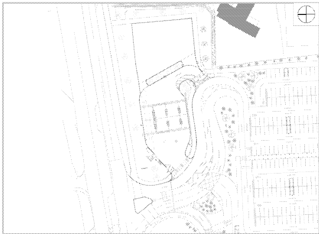
Figure 3.1 : Proposed PFS Layout (Courtesy of C+A Design)
