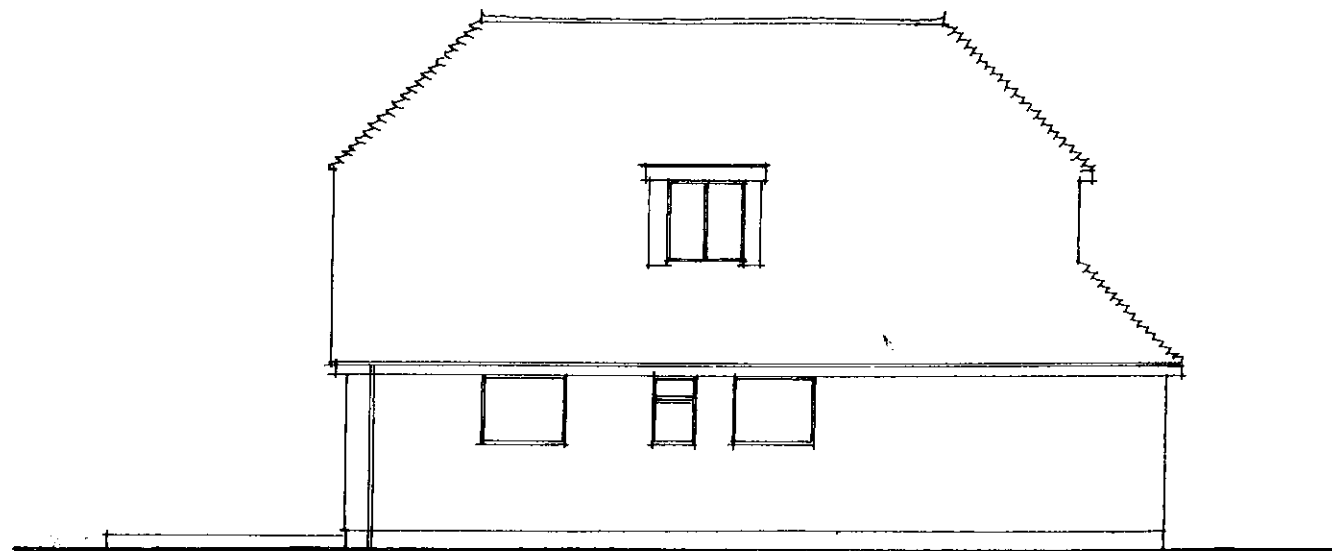
East Elevation
