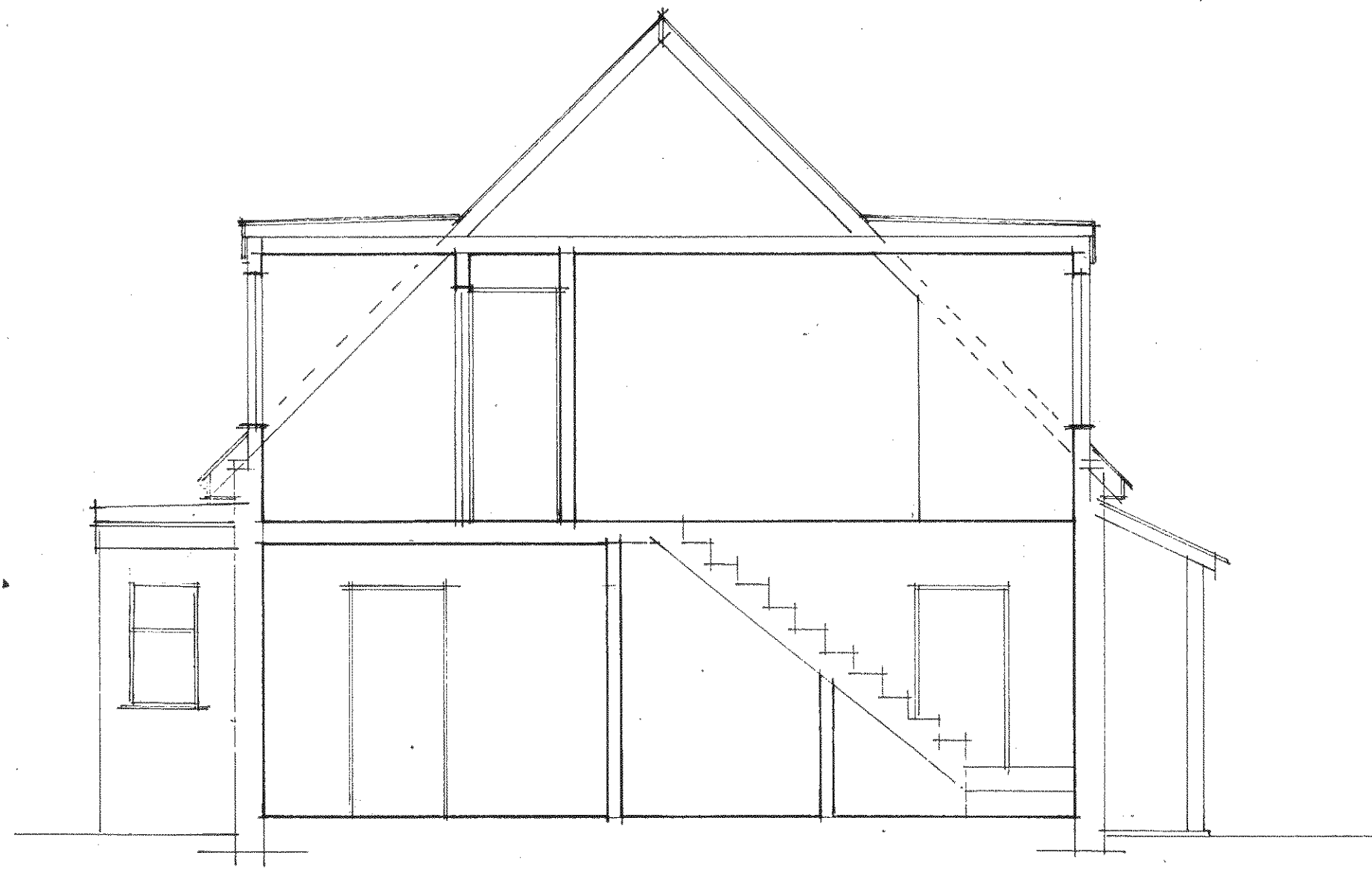
SECTION 1. EXISTING 1:50
