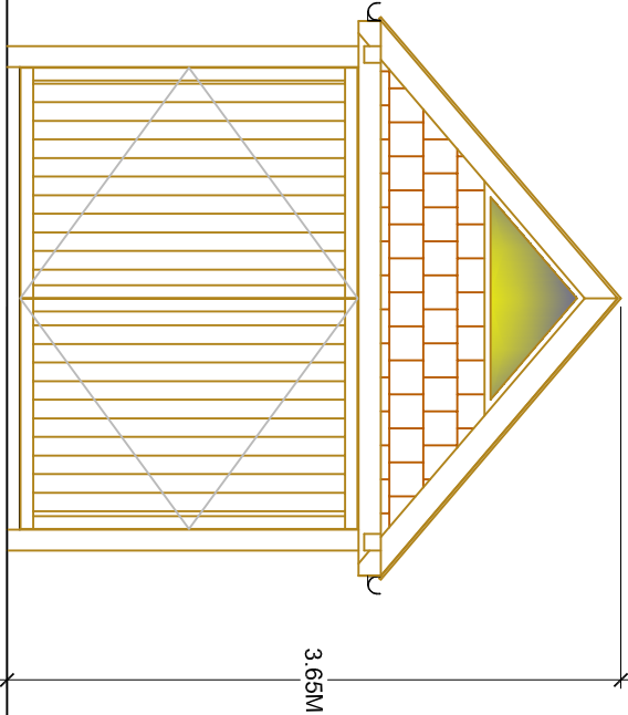
EAST ELEVATION
