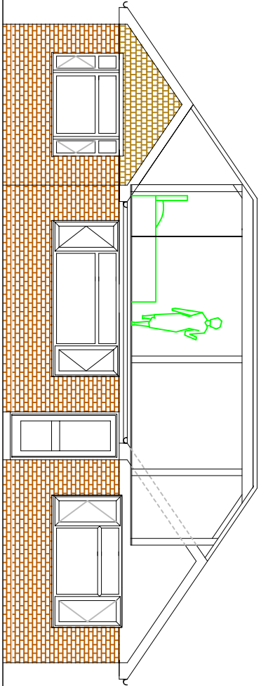
SCHEMATIC SECTION.
