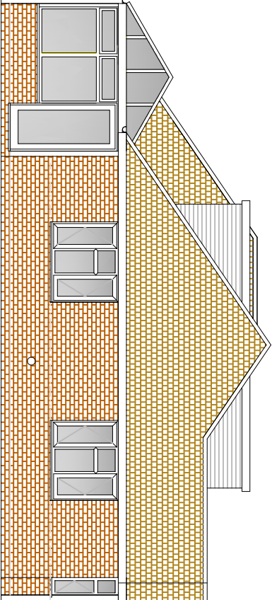
WEST ELEVATION
