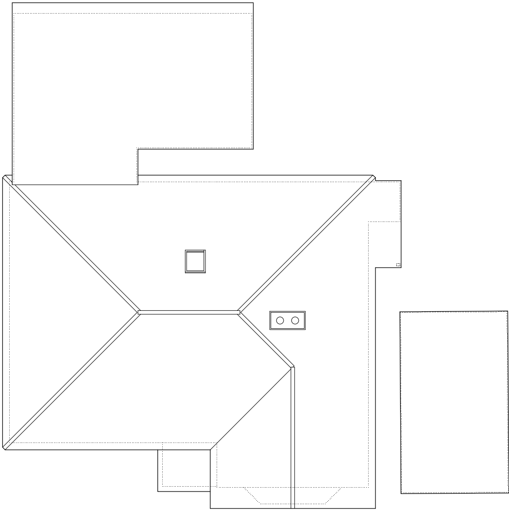
Roof Plan
