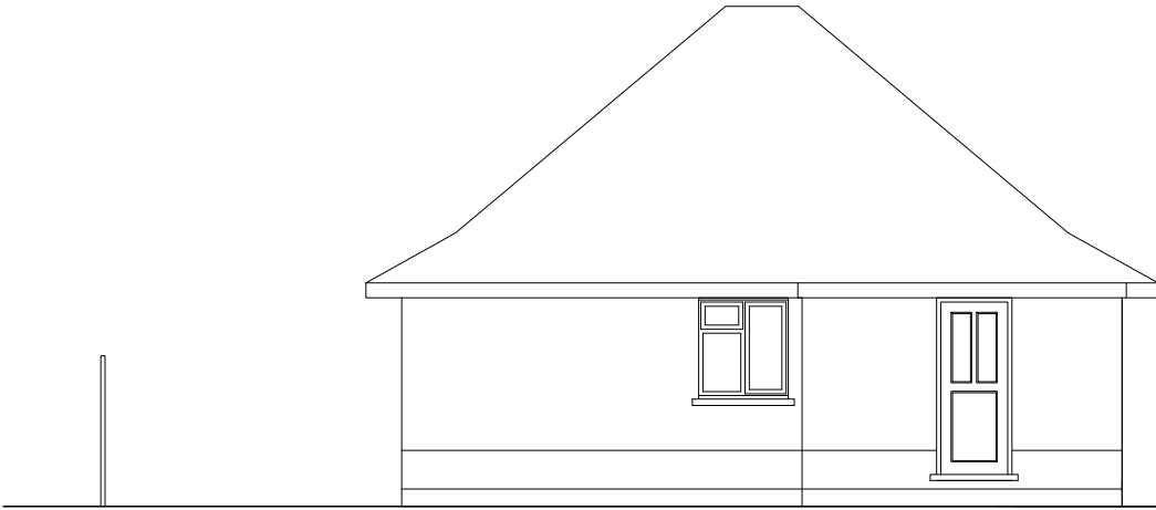
REAR ELEVATION (NORTH)
