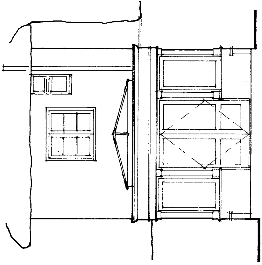
GARDEN ELEVATION
