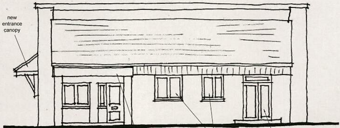
SOUTH ELEVATION
