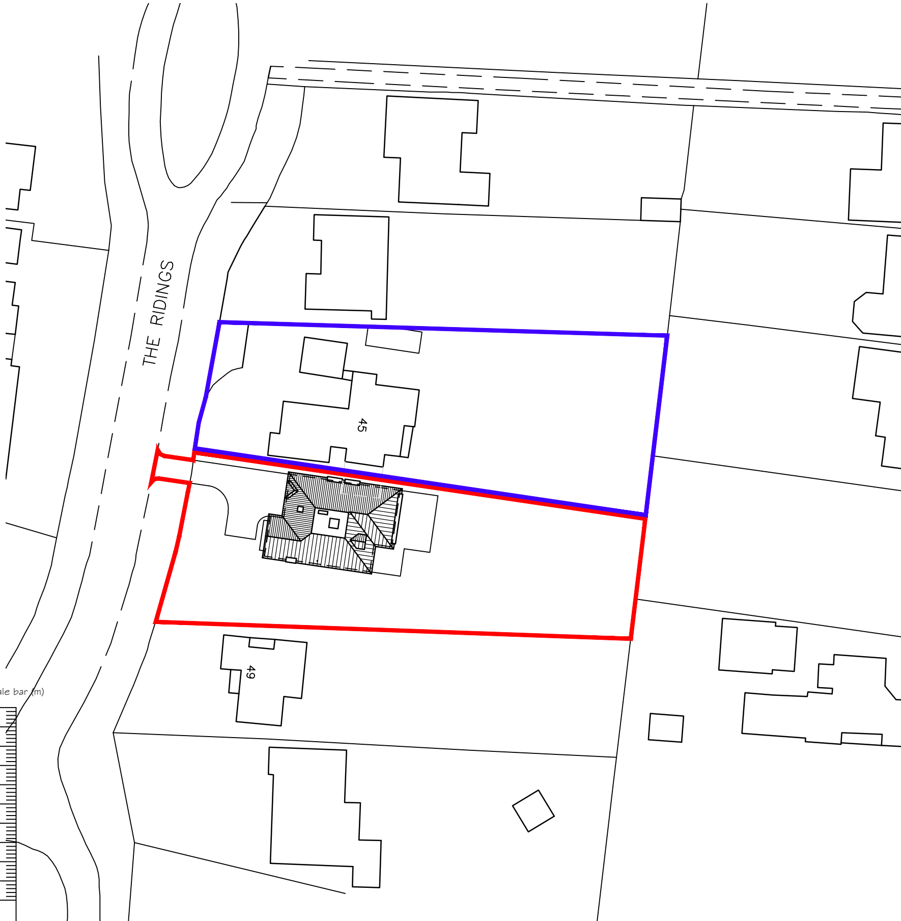
BLOCK PLAN 1:500
