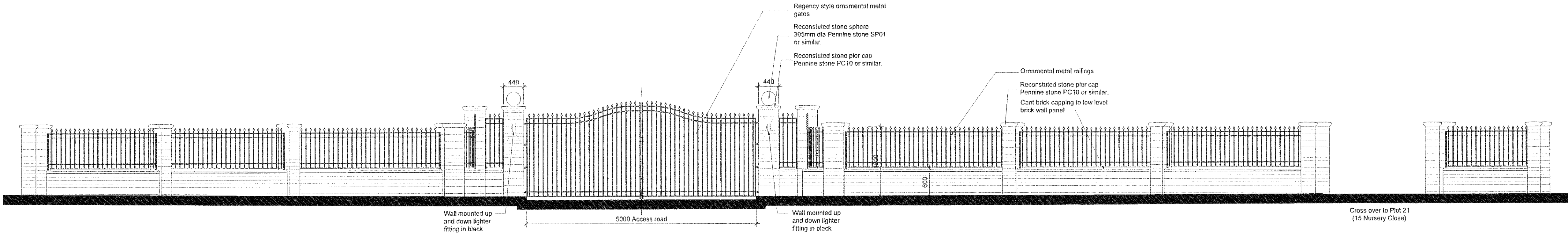
Elevation to Nursery Close 1:50
