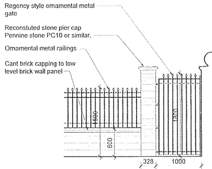
Pedestrian Access Gate Elevation 1:50
