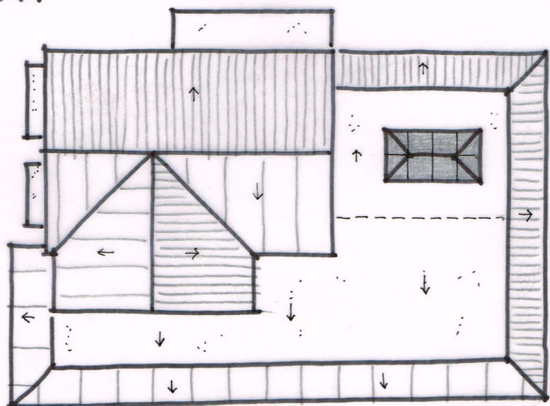
ROOF PLAN 1:200
