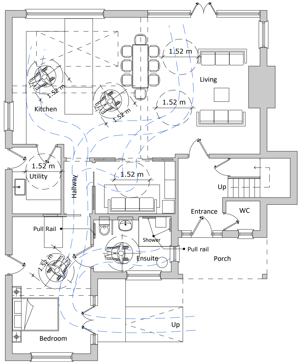
A :: Wheelchair Swept Path 03 scale: 1:100
