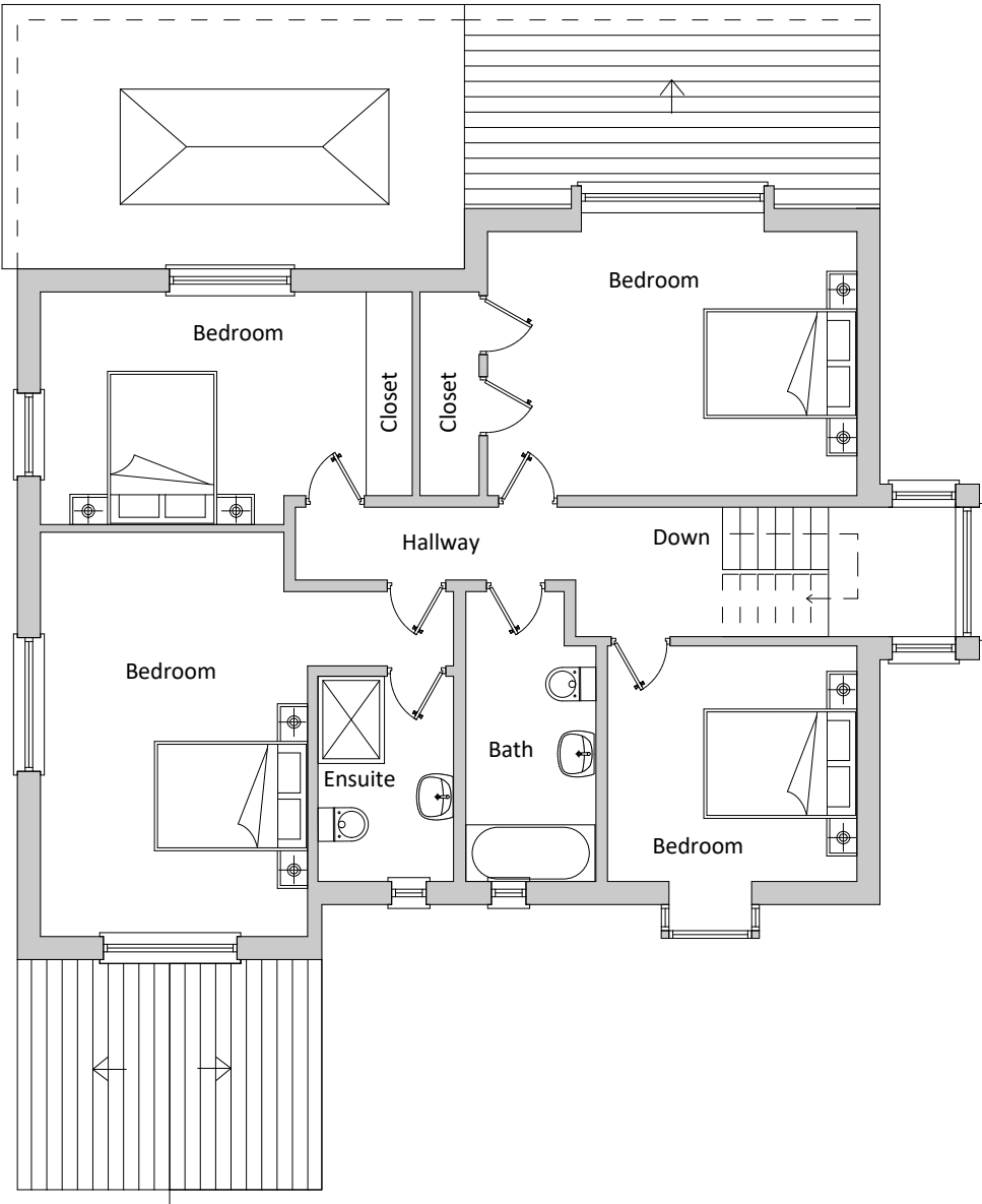
A :: Proposed First Floor Plan 02 scale: 1:100
