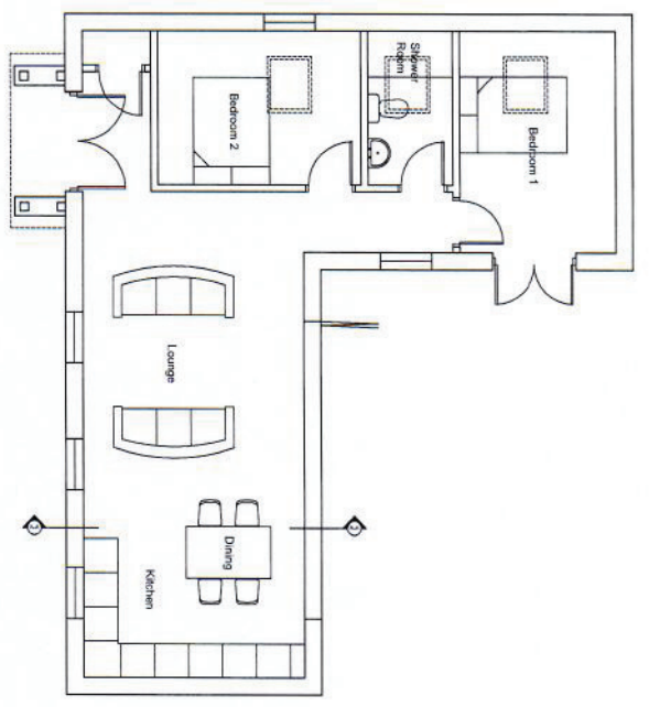
Plot 2: Ground Floor Plan
