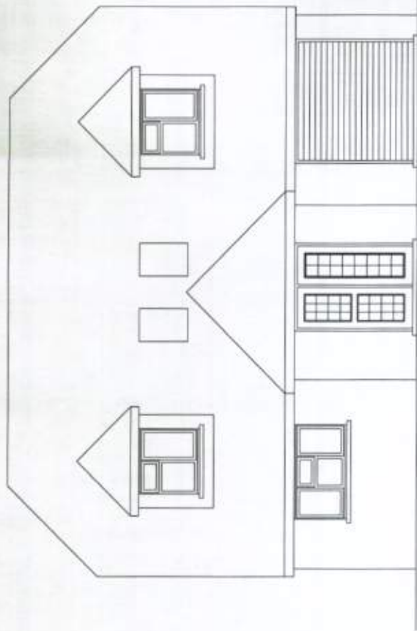
FRONT ELEVATION (NORTH).
