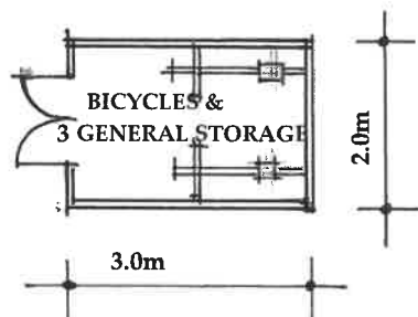
TYPICAL SHED PLAN
