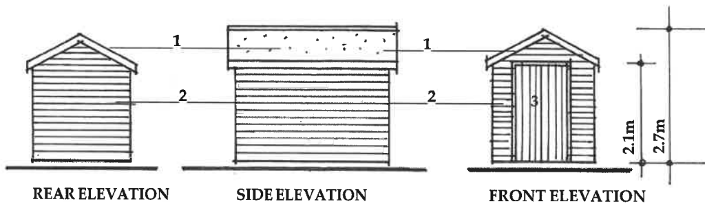
SIDE ELEVATION
