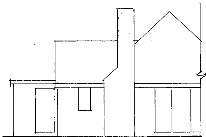
EXISTING SIDE ELEVATION (4)
