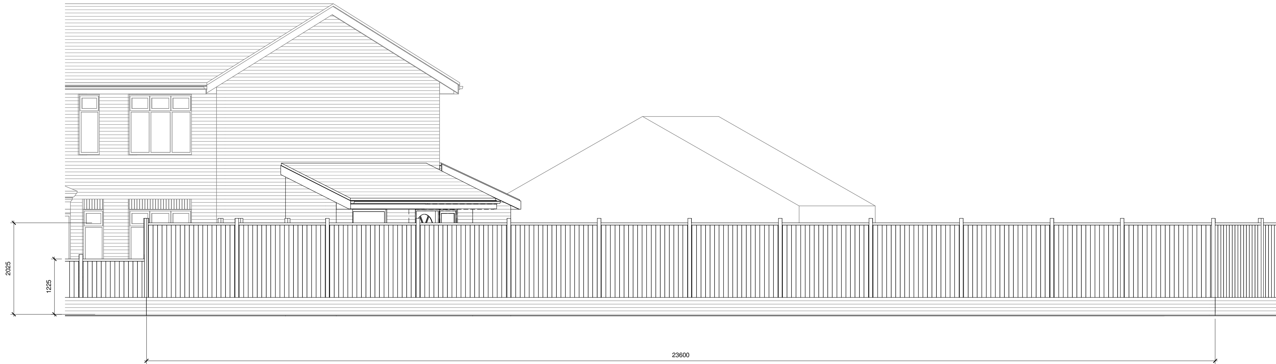
1 Fence Elevation 1 1 : 50
