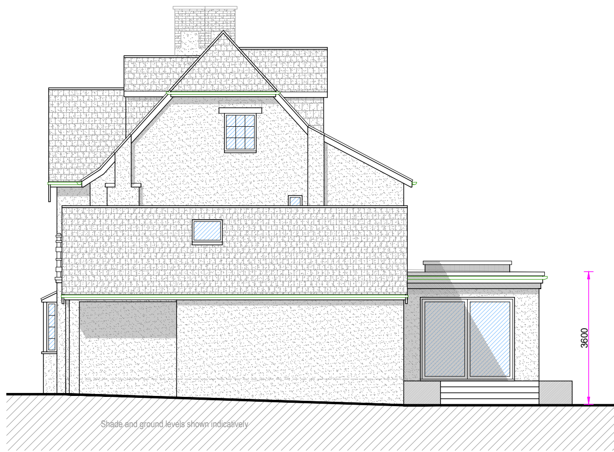
Right Side Elevation (Proposed)
