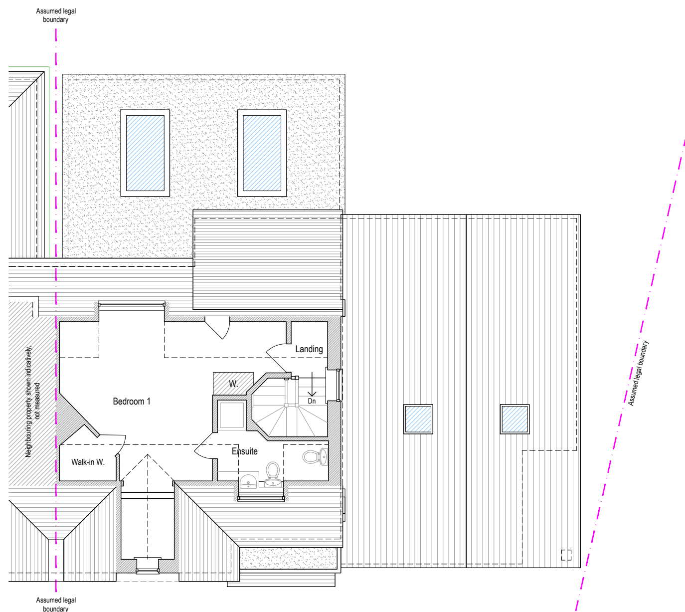
Second Floor Plan (Proposed)
