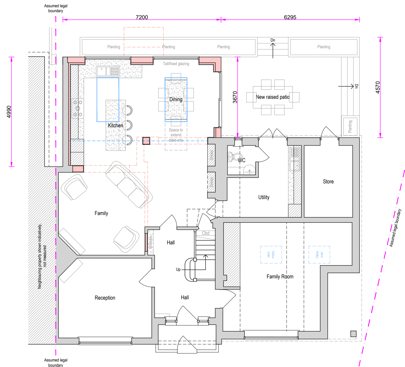
Ground Floor Plan (Proposed)
