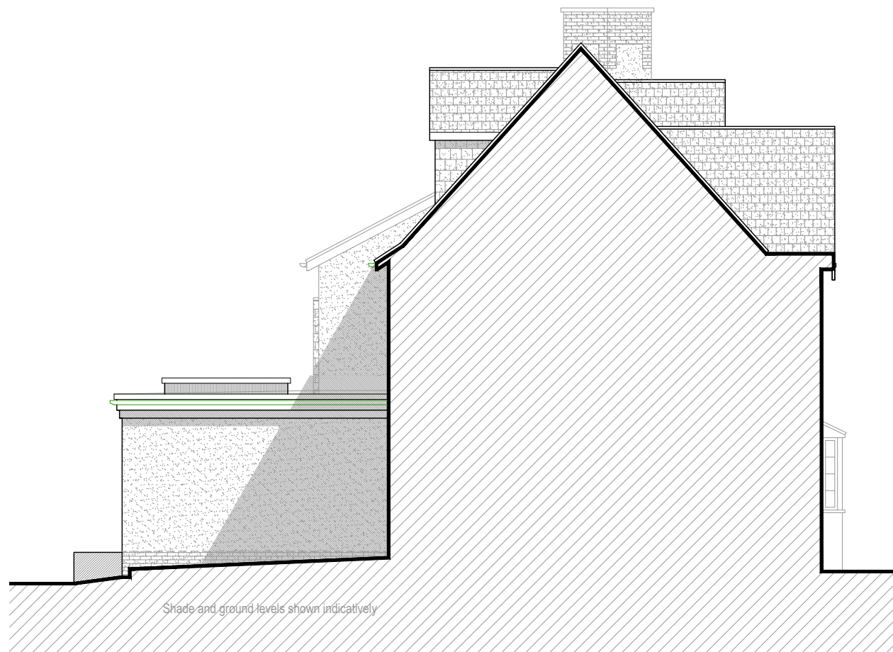
Sectional Left Side Elevation (Proposed)
