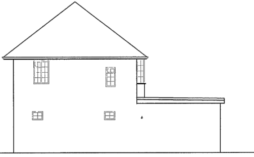
EXISTING WEST ELEVATION
