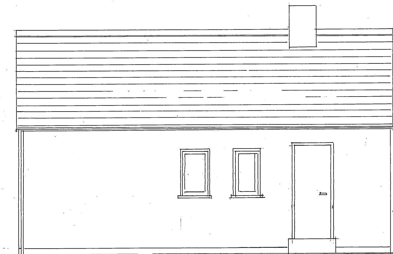
SOUTH ELEV
