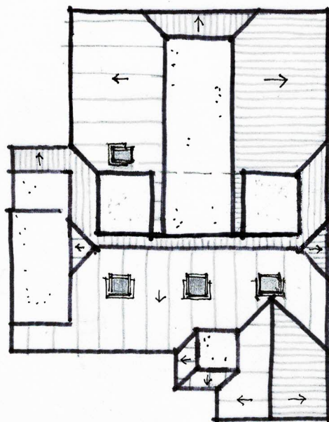
ROOF PLAN 1:200
