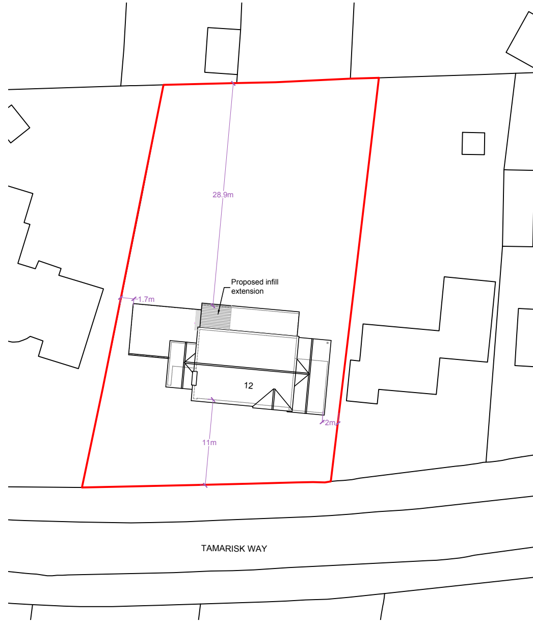
Block Plan 1:500
