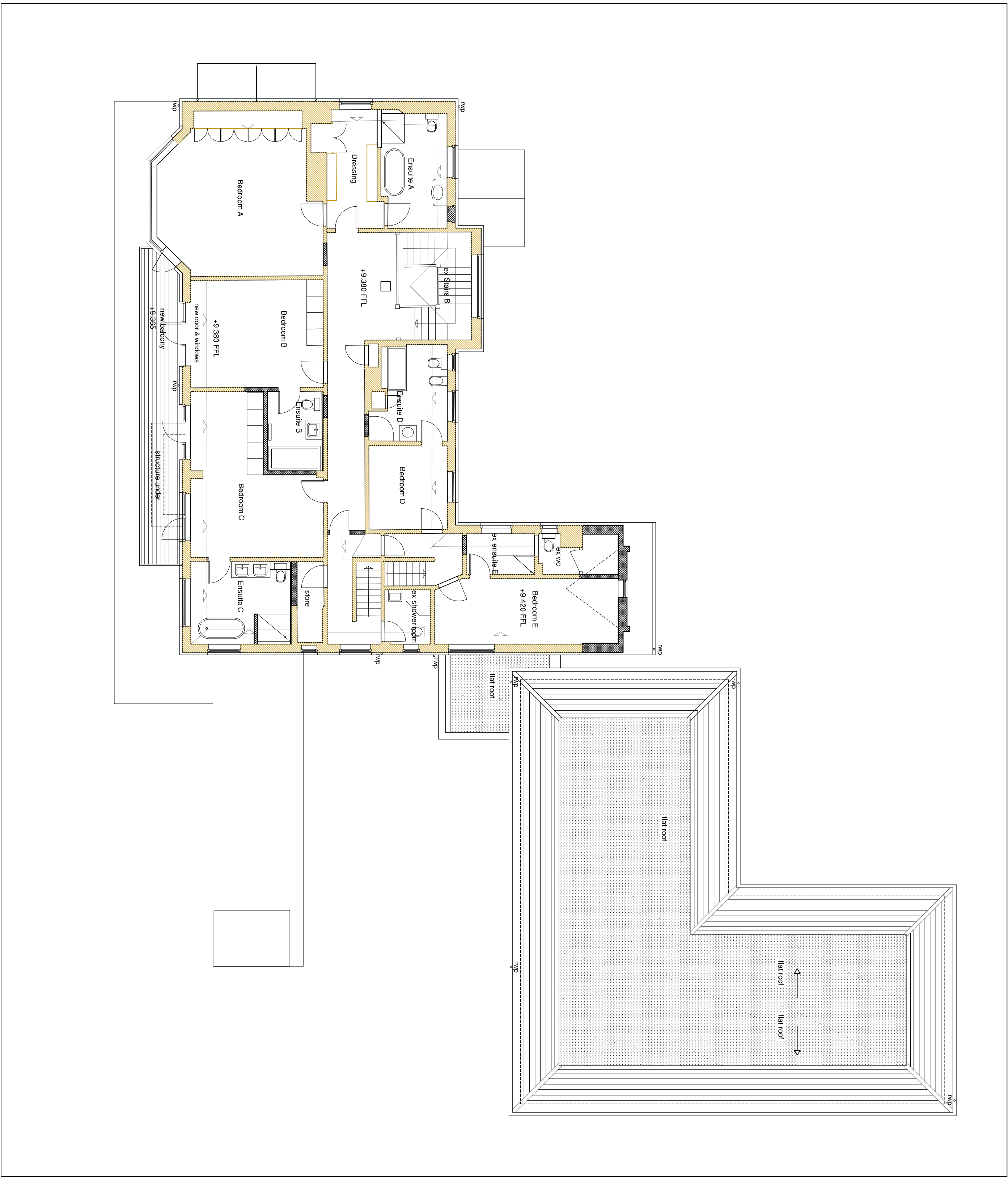
1:100 First floor plan as proposed
