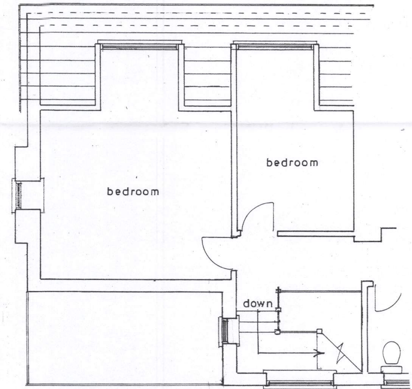
1st floorplan
