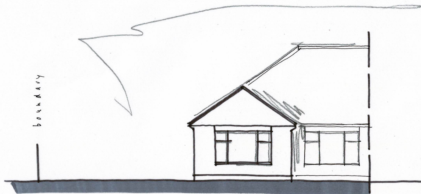
FRONT (s) ELEVATION 1:100 @ A3
