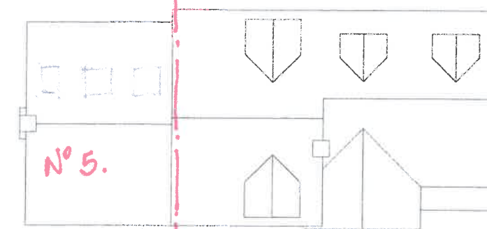
Roof Plan (1:100)
