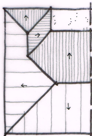
ROOF PLAN 1:200
