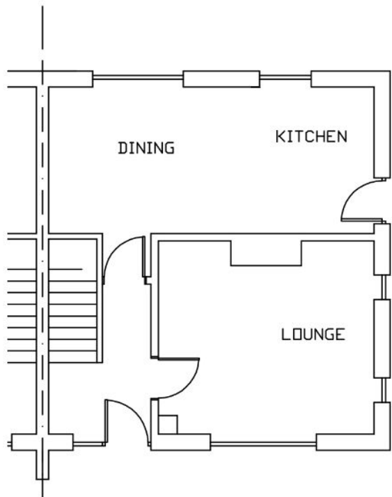
PROPOSED GROUND FLOOR PLAN 1/100
