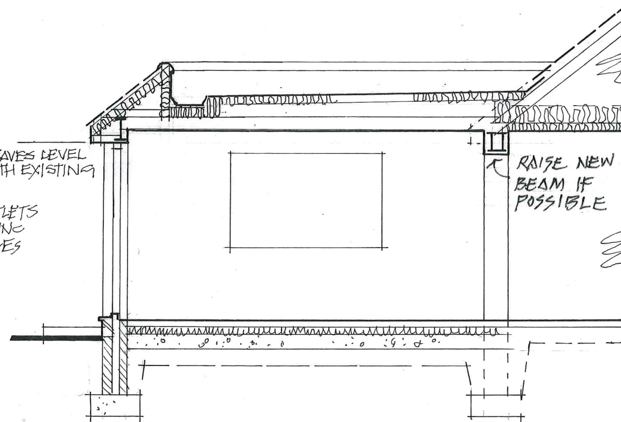
DIAGRAMMATIC SECTION THRU EXTENSION
