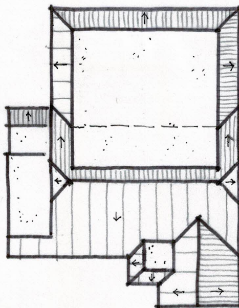
ROOF PLAN 1:200
