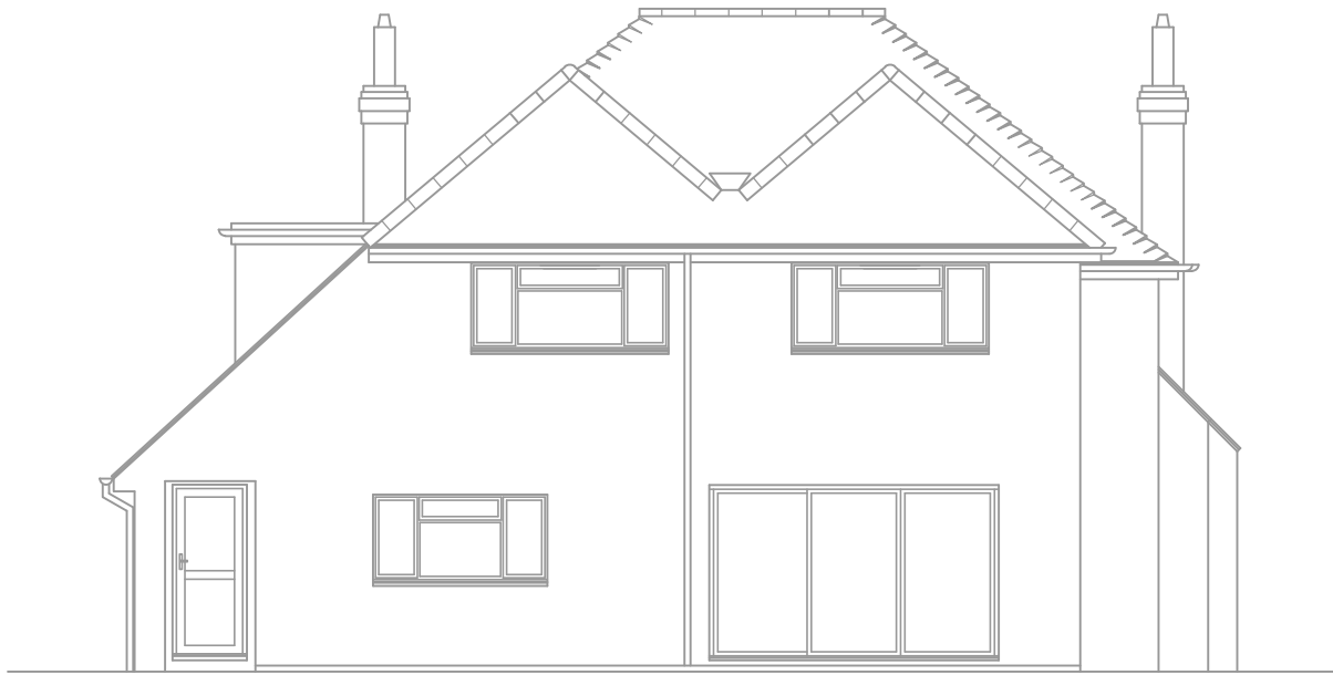
West Elevation – (Rear) 1:100
