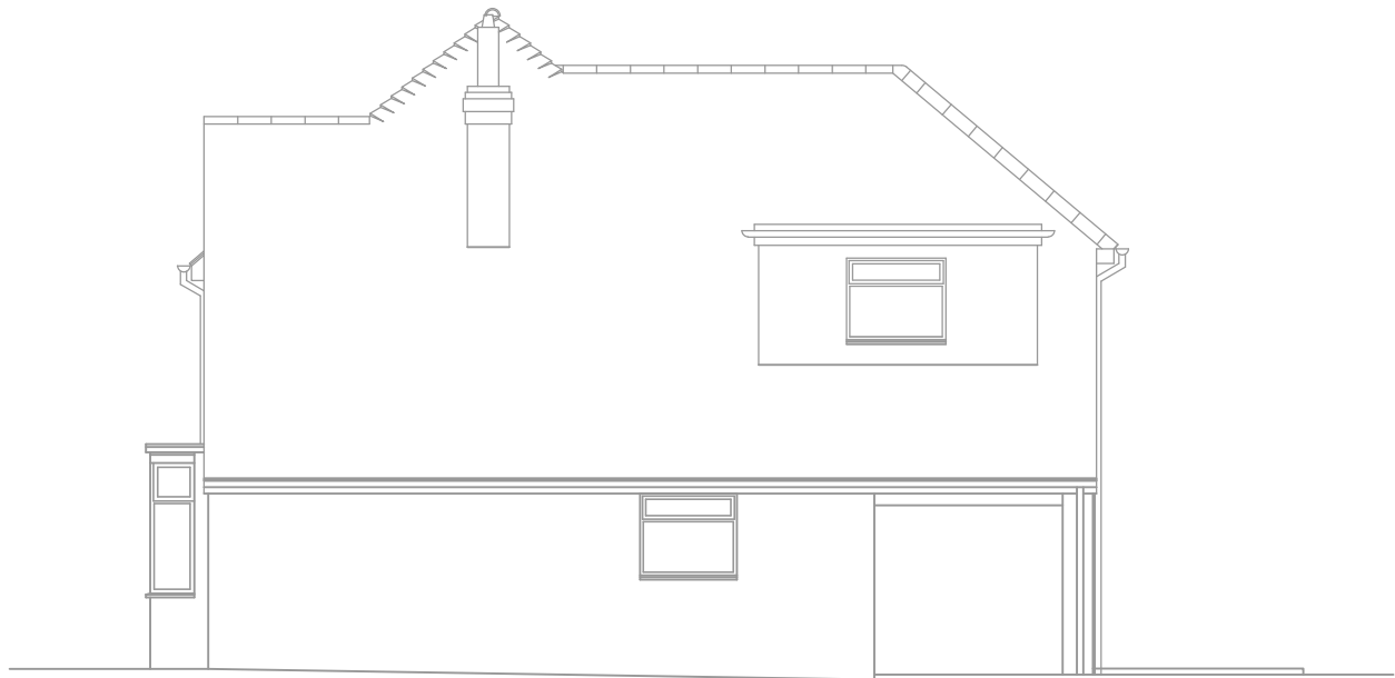
North Elevation – (Side) 1:100
