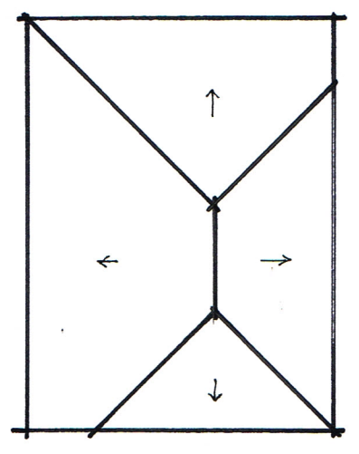
ROOF PLAN 1:100
