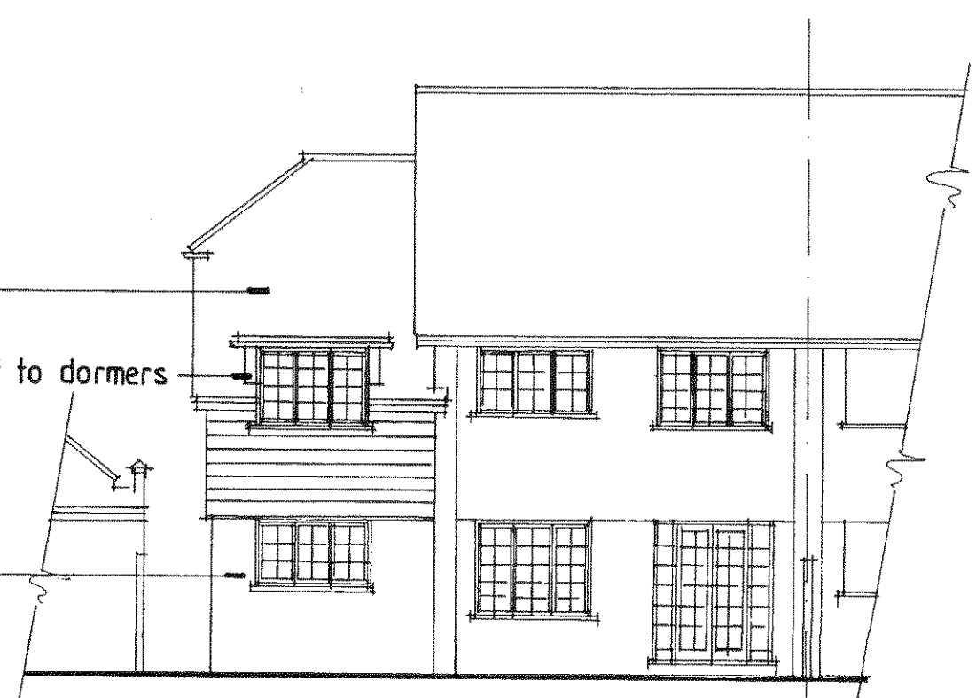
South elevation
