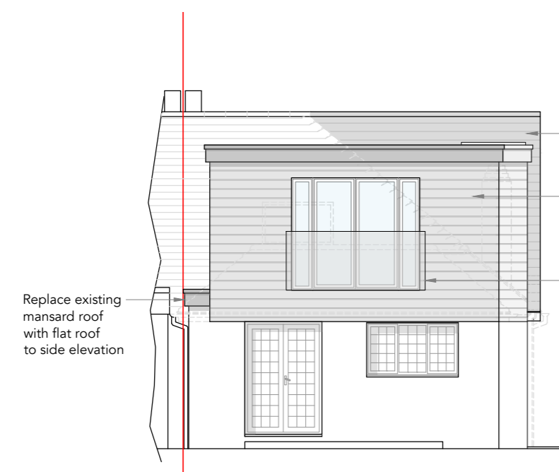
North Elevation (Rear) 1:100
