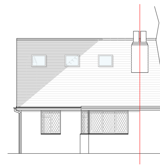
South Elevation (Front) 1:100
