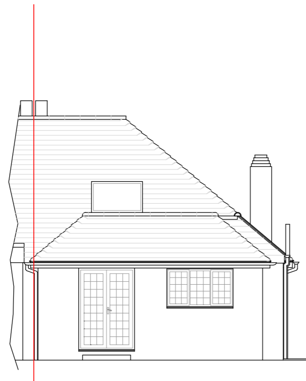
North Elevation (Rear) 1:100
