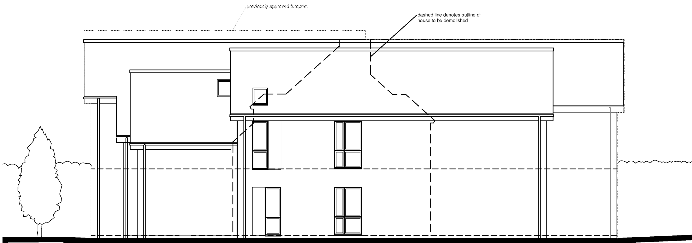
Comparison Western Elevation
