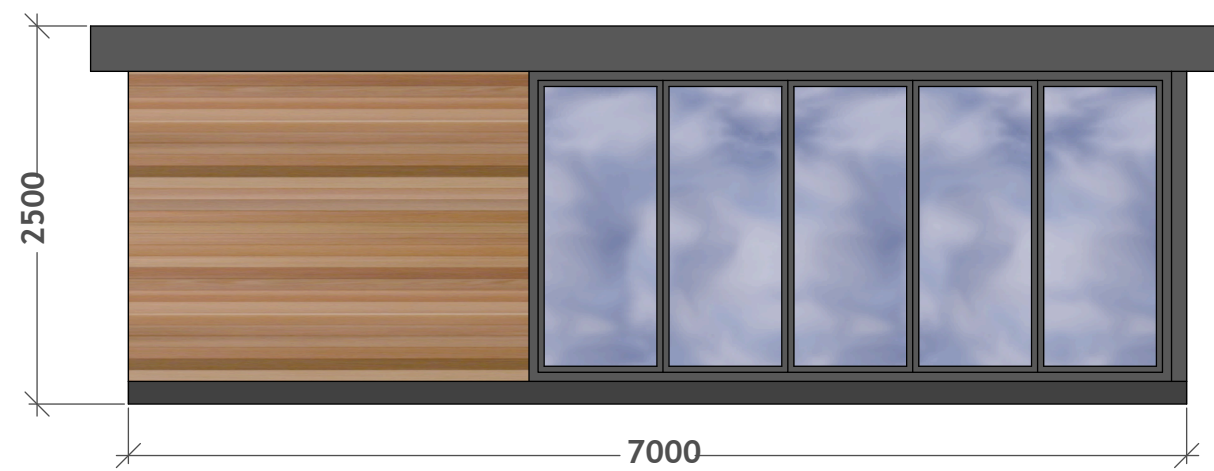
FRONT
